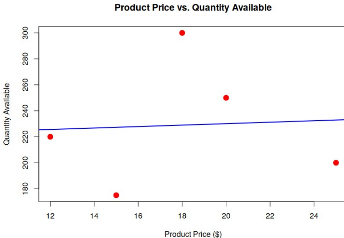
Output 4: Product Price vs Quantity Available Scatter Plot
